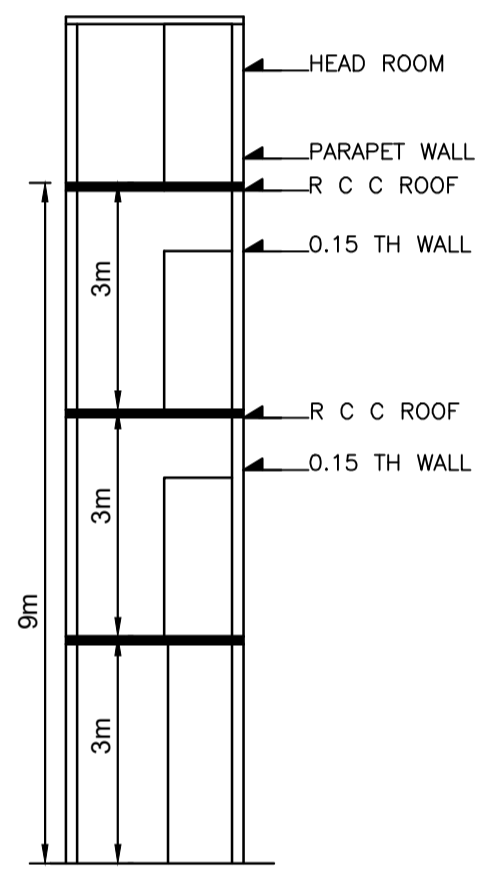
SECTION @X-X
